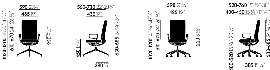
ID Soft L with fixed ring armrests
