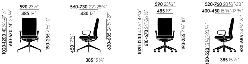
ID Soft L with height-adjustable ring armrests
