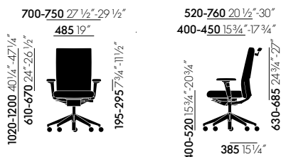
ID Soft L with 2D armrests and coat hanger
