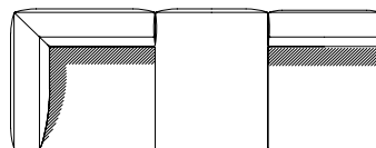
ART. DTLPT280 DX/SX L/W 280 H 82 P/D 100 W 110,2" H 32,3" D 39,4"
