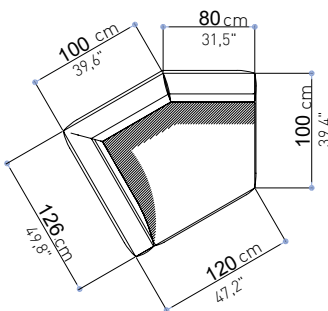
ART. DTLT168 DX/SX L/W 168 H 82 P/D 163 W 66,1" H 32,3" D 64,2"
